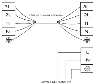
EACU-18 H/UP2/N3,
