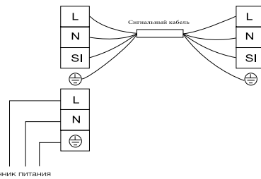
EACU-24 H/UP2/N3
